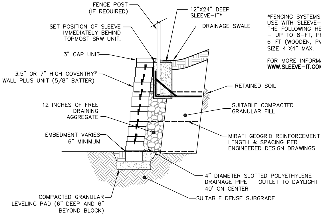
TYPICAL SECTION
