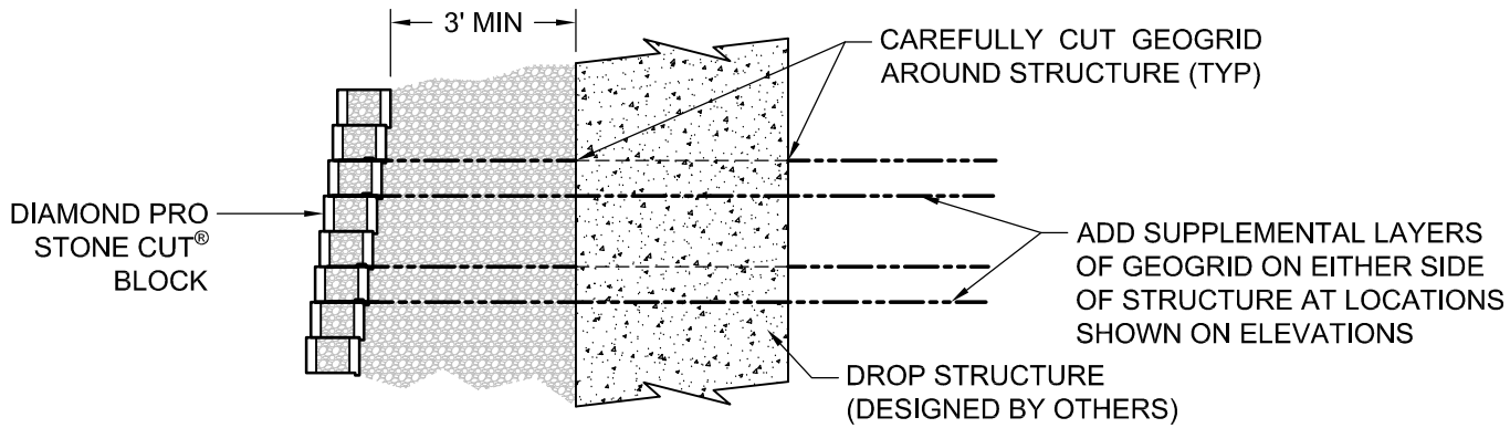
SECTION VIEW
