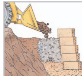
Dia. 7 – Compaction
