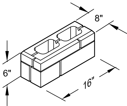
CAST STONE WALL CORNER UNIT
