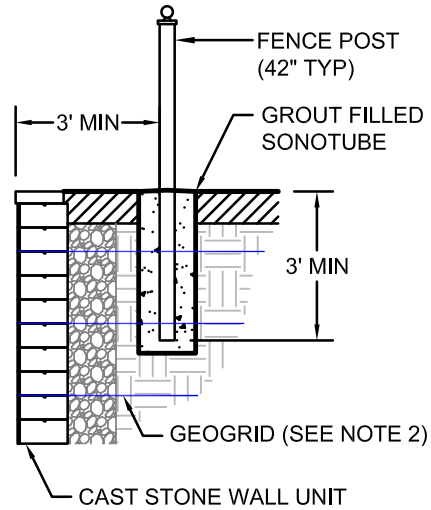
1 / 1 FENCE POST WITH SONO-TUBE
