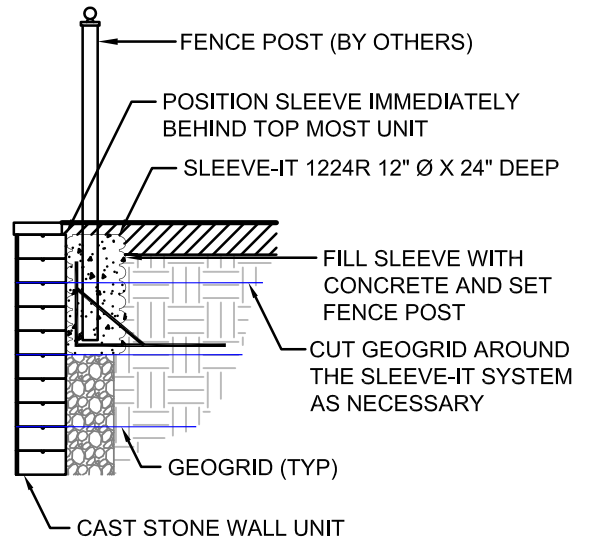
2 / 1 FENCE POST WITH SLEEVE-IT 1224R
