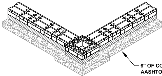
COURSE 1 PATTERN ISOMETRIC VIEW
