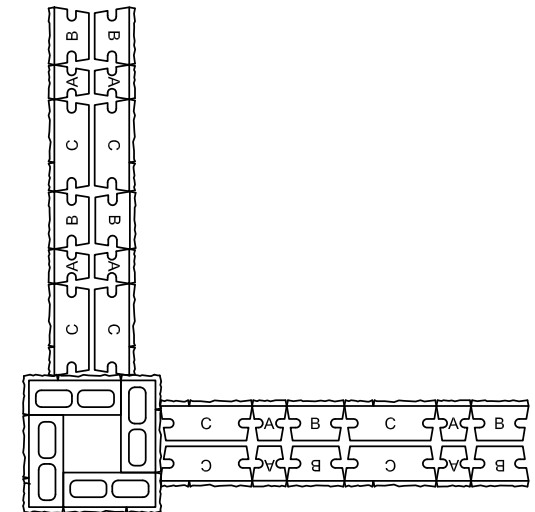
REPEAT COURSE 1 PATTERN PLAN VIEW
