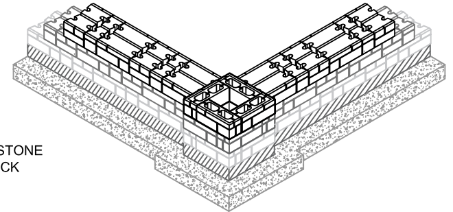
REPEAT COURSE 1 PATTERN ISOMETRIC VIEW
